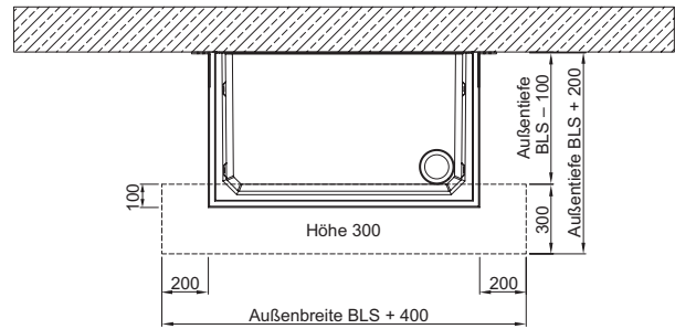
Fundament Option 2
