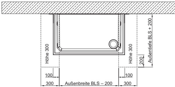
Fundament Option 1
